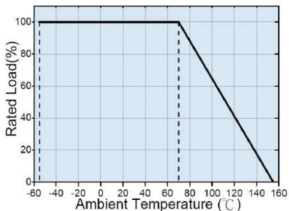
● POWER GRAPH
