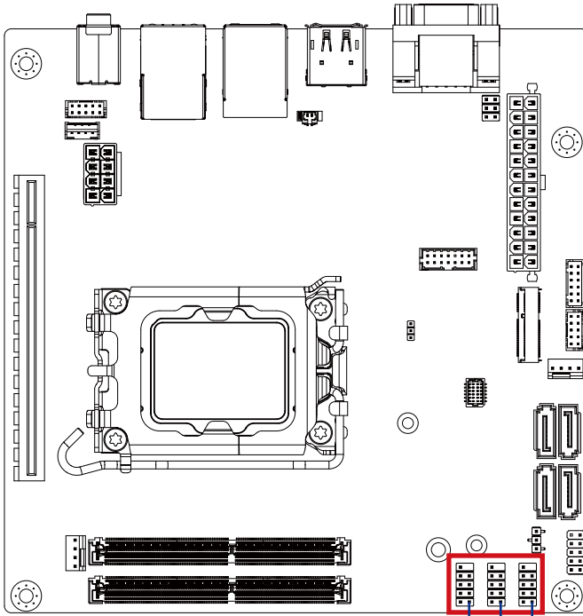
USB 2.0 Header
