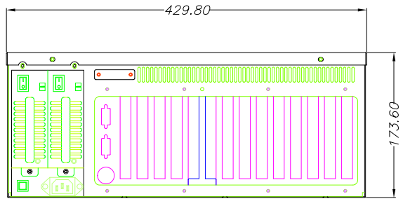
Rear view
