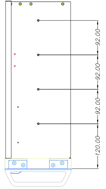
Right-side View
