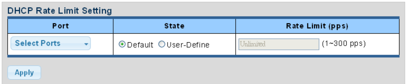
Figure 4-13-6-10: DHCP Rate Limit Setting Page Screenshot
