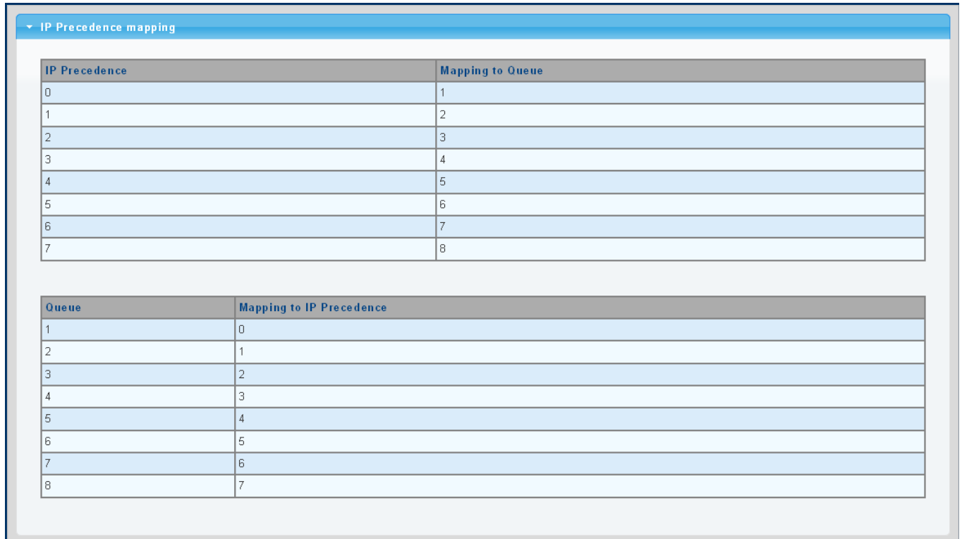
Figure 4-12-2-12: IP Precedence Mapping Page Screenshot
