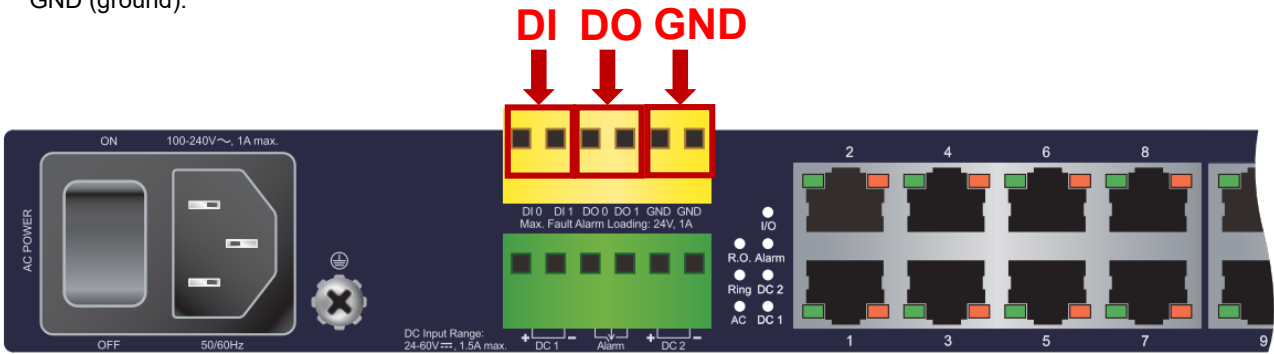
Figure 2-1-7-1 Wiring Digital Inputs/Outputs
